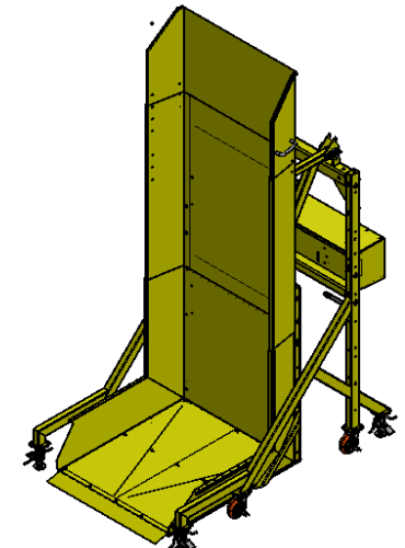
100 Inch Dump Over Configuration
