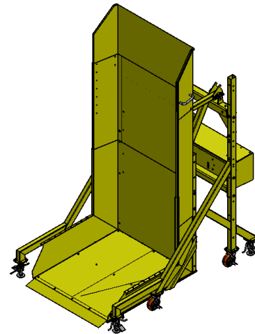
84 Inch Dump Over Configuration
